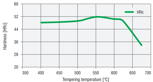
Tempering curve
