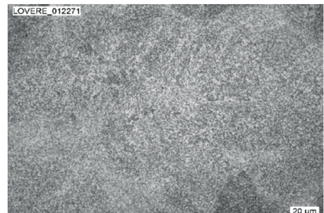
500x - Globular perlite with carbides
